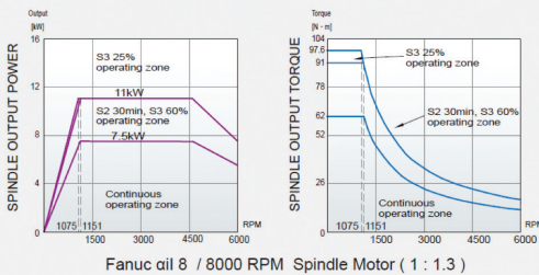
Fanuc oil 8 / 8000 RPM Spindle Motor ( 1 : 1.3 )
